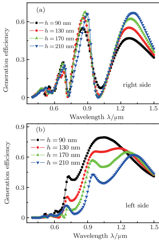
Fig. 7. (color online) Generation efficiency of the enhanced unidirectional SPPs generators with different h : (a) the right-going SPPs, (b) the left-going SPPs.
