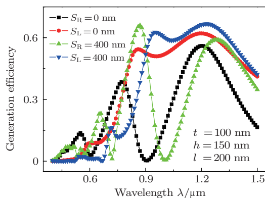
Fig. 3. (color online) Generation efficiency of the left-going and right-going SPPs for the regular unidirectional SPPs generators and the enhanced unidirectional SPPs generators.
