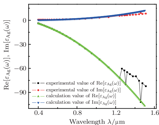
Fig. 2. (color online) Experimental values and calculated values of the silver permittivity.
