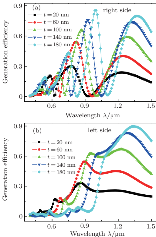
Fig. 8. (color online) Generation efficiency of the enhanced unidirectional SPPs generators with different t : (a) the right-going SPPs, (b) the left-going SPPs.
