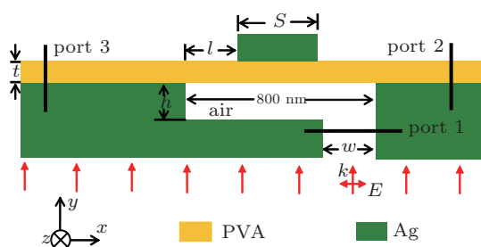
Fig. 1. (color online) Schematic of the enhanced unidirectional SPPs generators.
