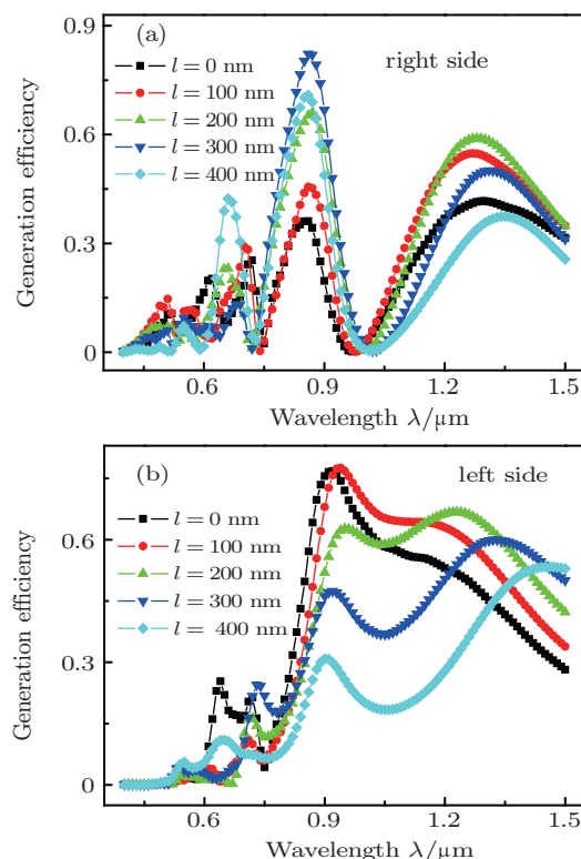
Fig. 6. (color online) Generation efficiency of the enhanced unidirectional SPPs generators with different l : (a) the right-going SPPs, (b) the left-going SPPs.
