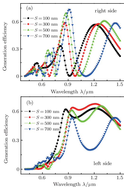
Fig. 5. (color online) Generation efficiency of the enhanced unidirectional SPPs generators with different S : (a) the right-going SPPs, (b) the left-going SPPs.
